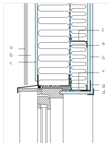
YU12: Overkant vindue
