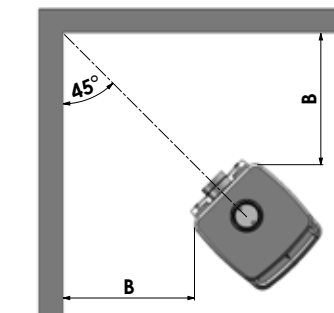
3112 corner installation
