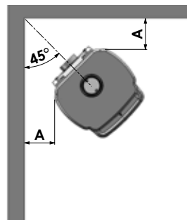
3142 corner installation
